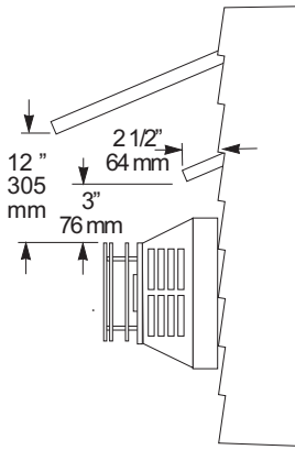
Figure 18. Wall Vent Terminal / Overhang Clearances
